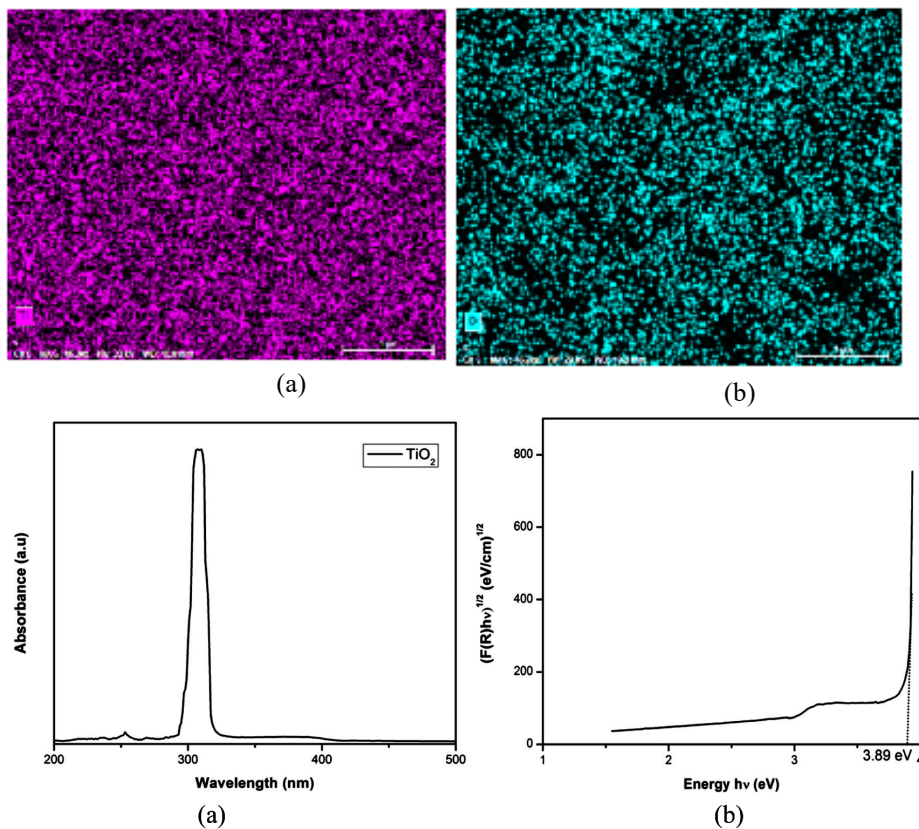
Figure 4: Elemental map of (a) Ti (b) O; & Absorption Spectrum and Tauc plot of TiO 2 thin film
